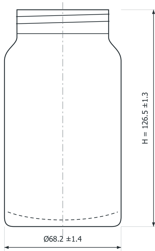
FRONT VIEW
