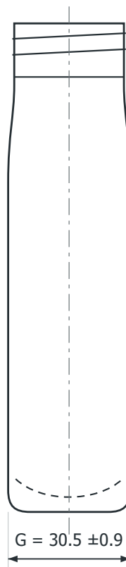
SIDE VIEW
