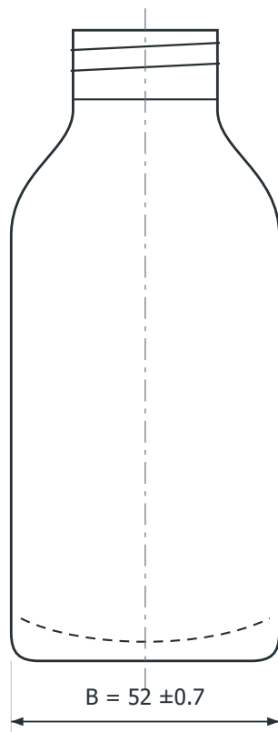
FRONT VIEW
